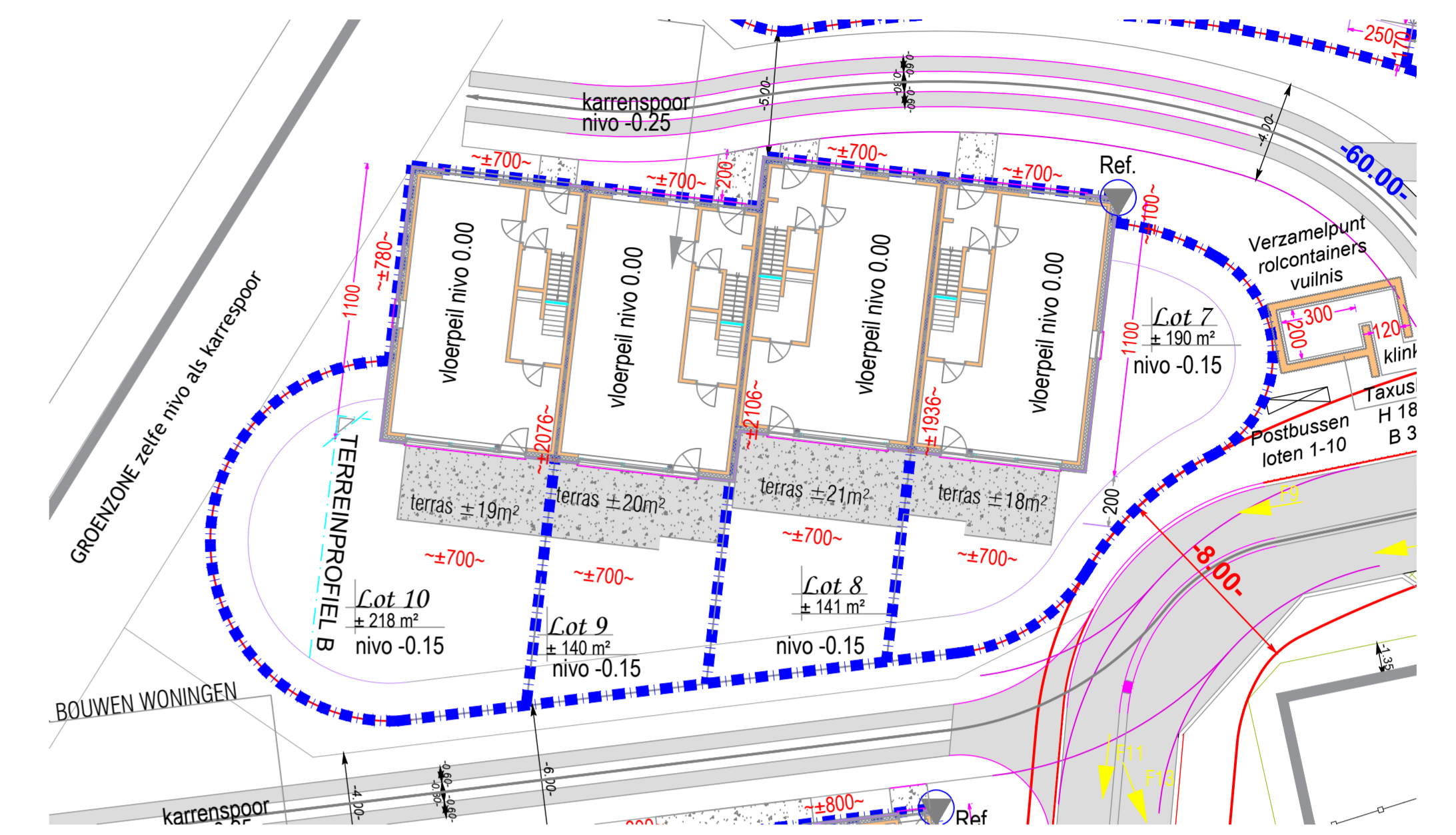
INPLANTING
